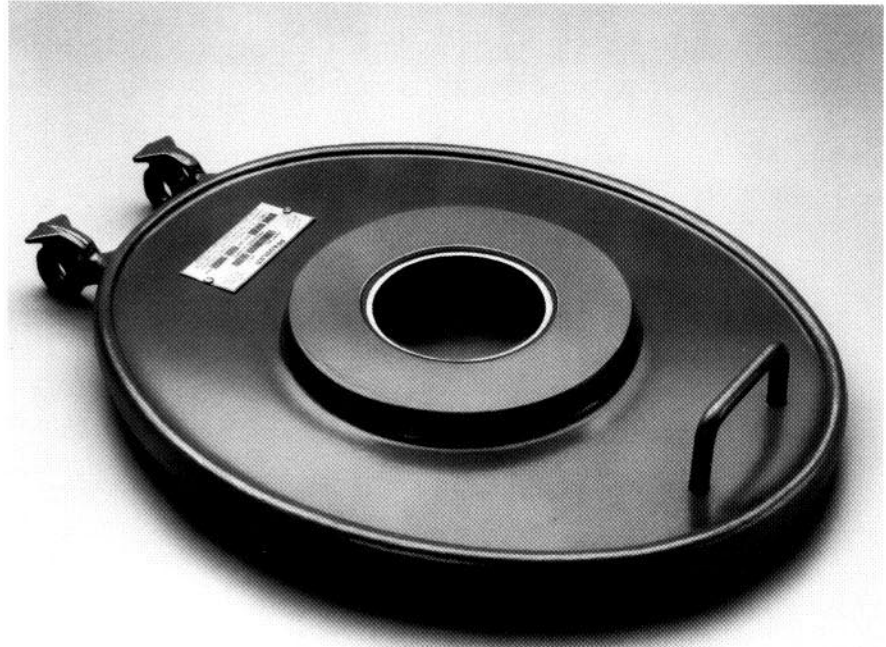
Pfaudler manway cover with integral fused-steel sight glass. Note smooth, clean exterior surface that results from eliminating the usual mounting flanges, gaskets, etc.
